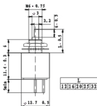
TOLERANCES: \pm 0.2 EXCEPT WHERE NOTED CE12STPM-P-5
