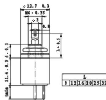
TOLERANCES: \pm 0.2 EXCEPT WHERE NOTED CE12STPM-P-3
