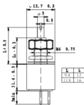
TOLERANCES: \pm 0.2 EXCEPT WHERE NOTED CE12STPM-B
