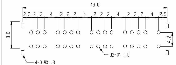
PCB LAYOUT
