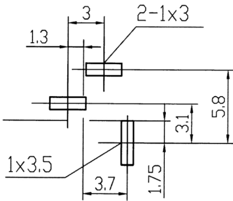
PCB Holes Diagram (VIEWED FROM COPPER SIDE)
