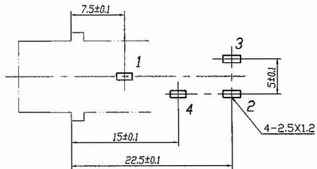
PCB MOUNTING HOLES (TOP VIEW)
