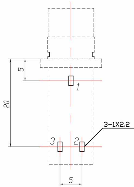
P.C.B Holes Diagram Bottom View
