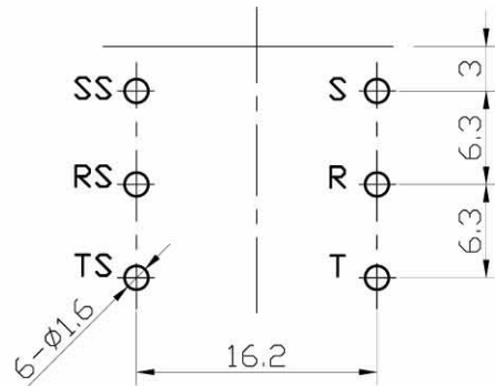
PCB MOUNTING HOLES (VIEWED FROM COPPER SIDE)
