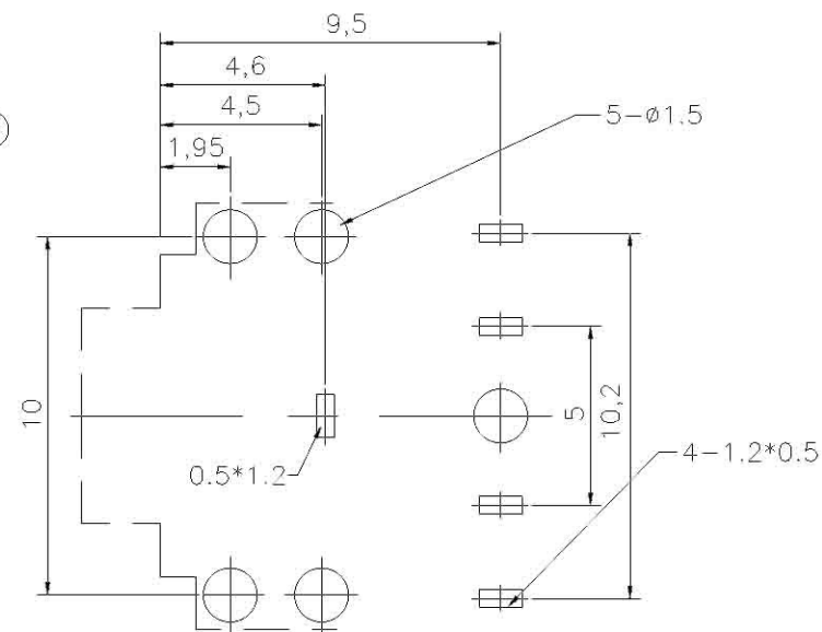
P.C.B. HOLE LAYOUT (BOTTOM VIEW)
