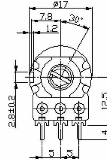
SHAFT SHOWN IN FULL C.C.W. POSITION
