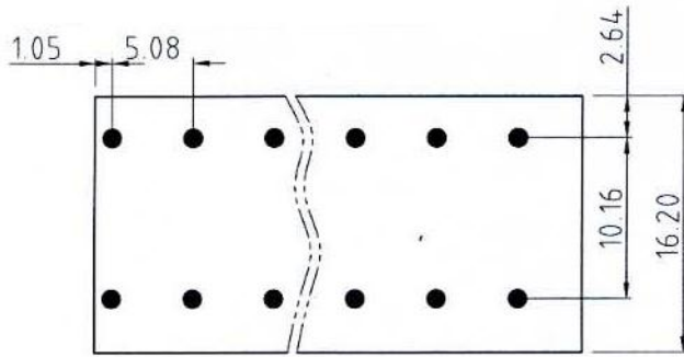
● FOR PIN P.C.B LAYOUT
