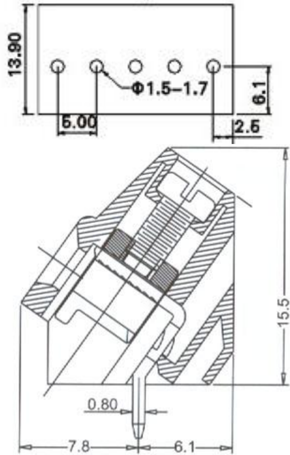
PCB Layout
